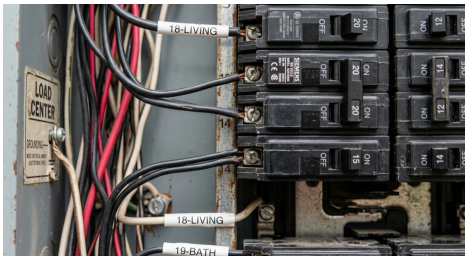
Panel interior, dead front removed
